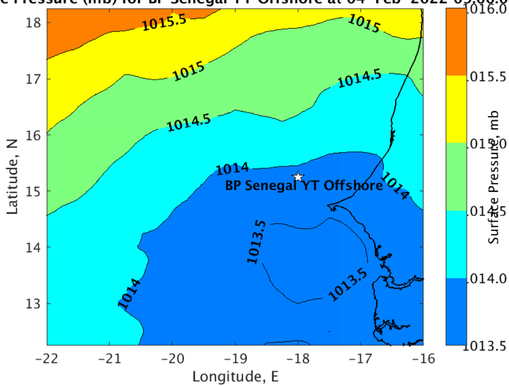
Surface Pressure (mb) for BP Senegal YT Offshore at 04-Feb-2022 09:00:00
